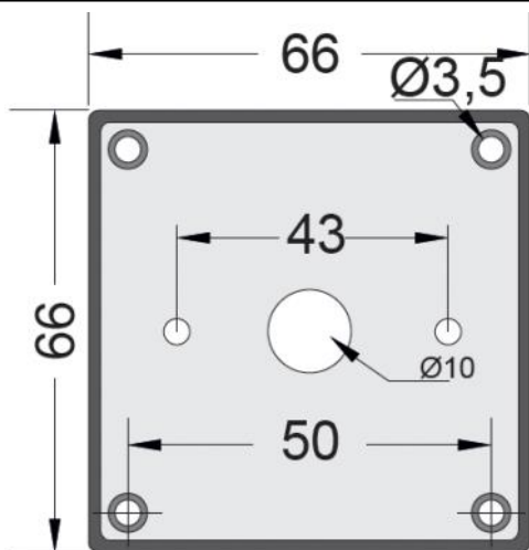
STANDARD FRAME
