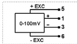
TRANSDUCER 0-100mV
