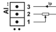
- Potentiometric transmitter
