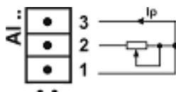
- Resistance transmitter
